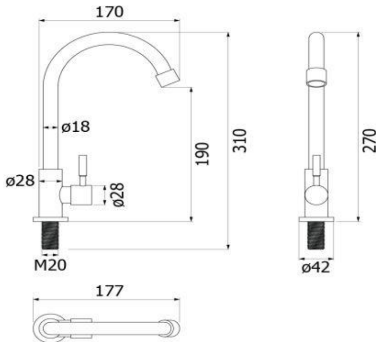
HFHOB-1000HY1 unit : mm
