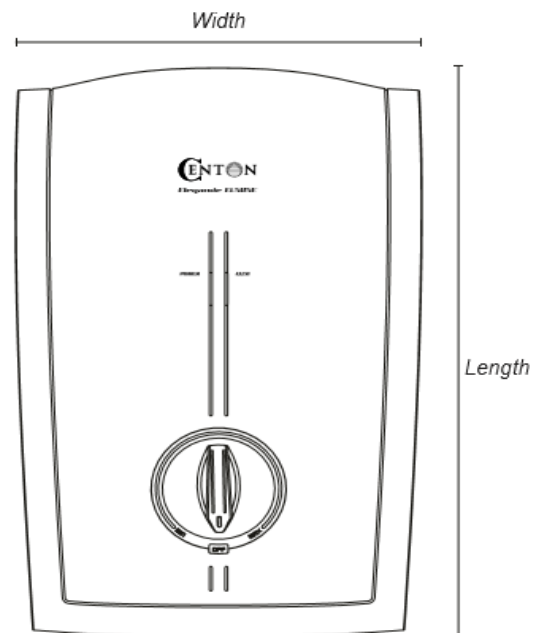
Elegande EL505 Heater Dimension: 209mm (W) x 326mm (L) x 91mm (H)
